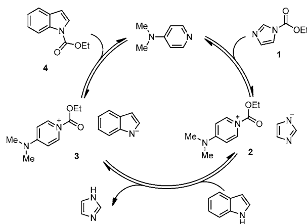
Scheme 1. Mechanistic hypothesis.
